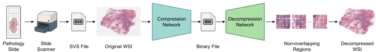
Fig. 1. The workflow of PathoLIC. Histology slides are digitized into WSIs in SVS format, which are partitioned into non-overlapping regions, each containing 16 patches. By exploiting patch-level correlations, the network reduces redundancy and yields a binary file significantly smaller than the original SVS. During decompression, PathoLIC restores the WSI with high fidelity, ensuring that fine-grained histological details are preserved.
