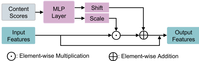
Fig. 3. Architecture of the proposed QCM. Content scores Q are mapped by an MLP to generate scale ( \alpha ) and bias ( \beta ) parameters, which modulate the input feature map via an affine transformation for content-aware compression.
